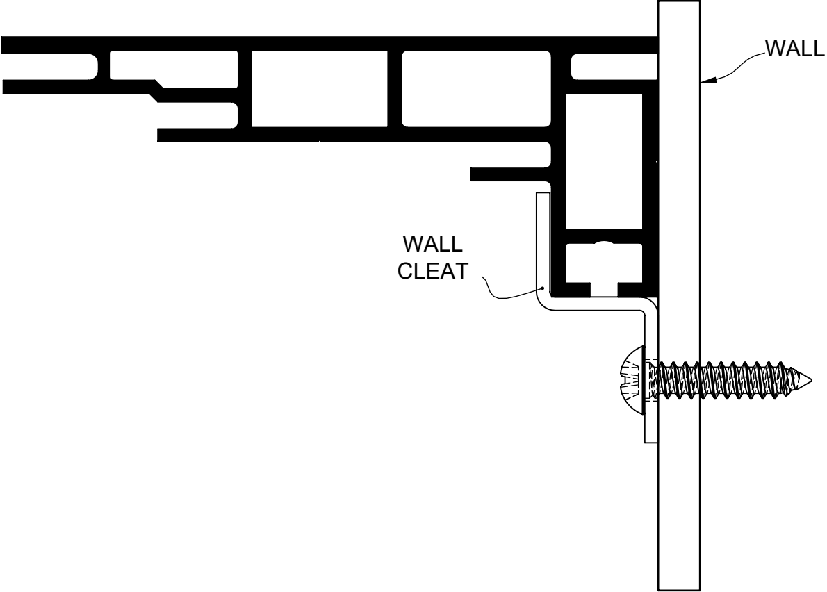
100MM SEG EXTRUSION
