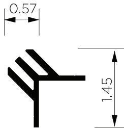
CORNER CLADDING
