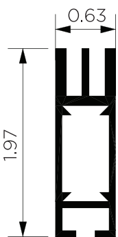
CUBE EXTRUSION
