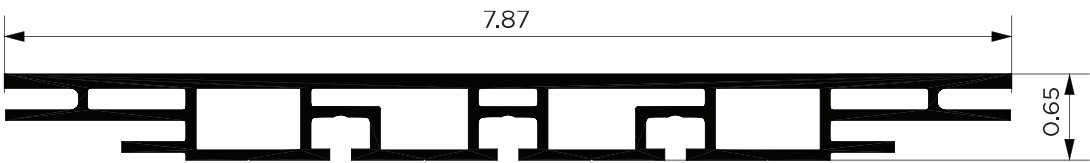
200mm SEG EXTRUSION (LIGHTBOX COMPATIBLE)
