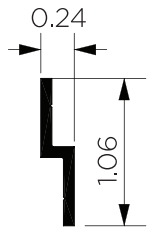
S SHAPE EXTRUSION
