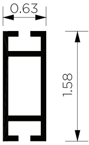
RAIL EXTRUSION
