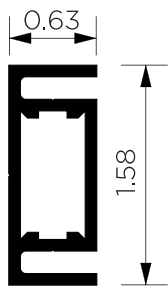
SEG SPREADER LIGHTBLANKET 140" RADIUS BEND
