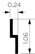
S SHAPE EXTRUSION
