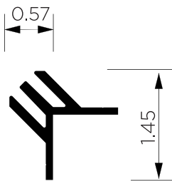
CORNER CLADDING
