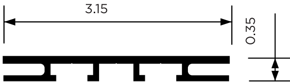
80mm SEG BENDABLE (LIGHTBOX COMPATIBLE)
