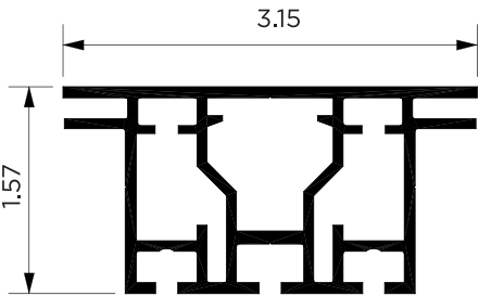
80mm SEG EXTRUSION
