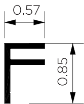
F SHAPE EXTRUSION
